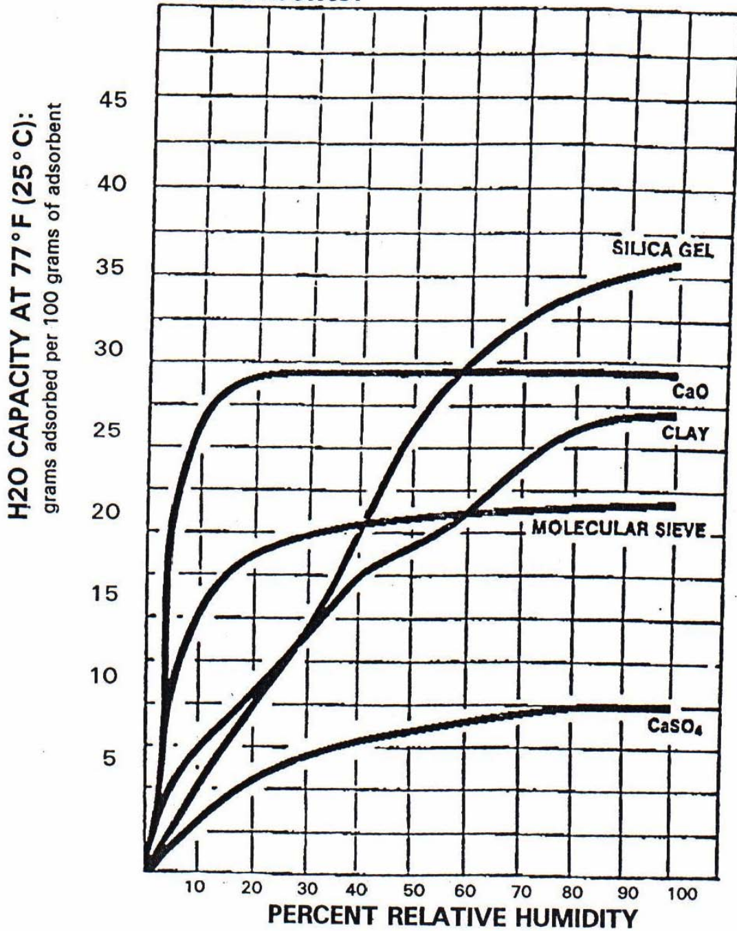
Figure 2: Equilibrium capacity (H 2 O) of various adsorbents.
