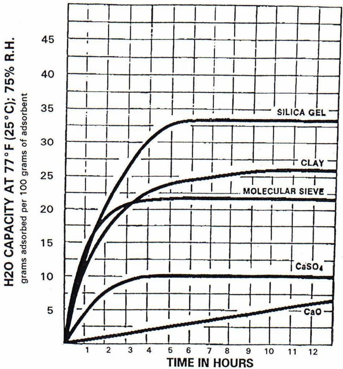
Figure 3: Adsorption rate(H 2 O) of various adsorbents.
